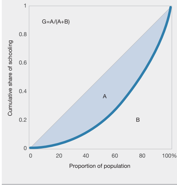
Figure 3.11 Hypothetical Lorenz Curve for years of schooling and Gini coefficient
