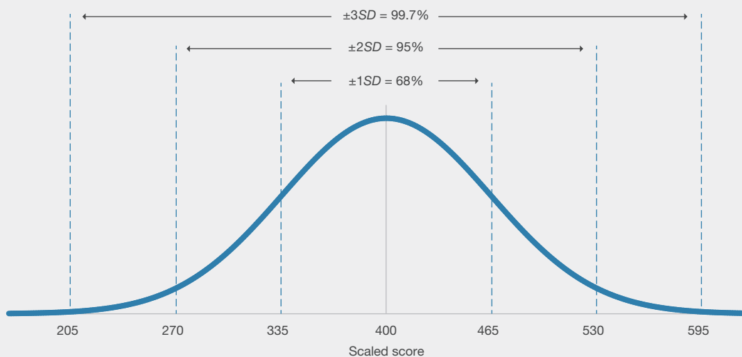
Figure 3.9 Gaussian distribution in relation to Chebychev's rule
