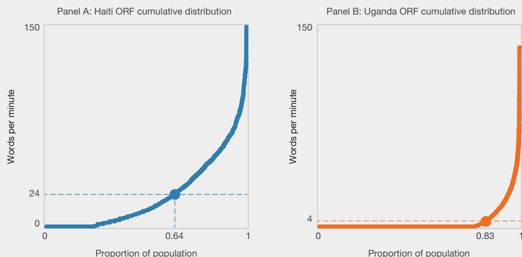
Figure 3.4 Empirical cumulative distributions of EGRA oral reading fluency (ORF) results for Haiti and Uganda
