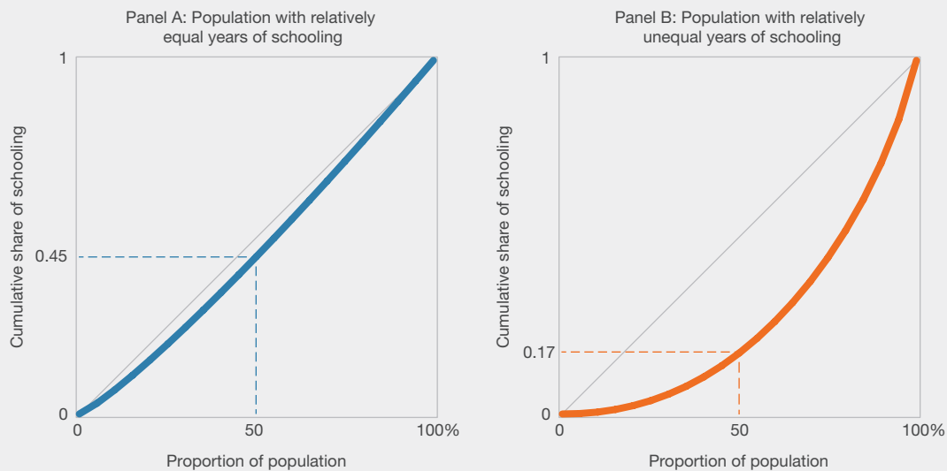
Figure 3.5 Hypothetical Lorenz curves illustrating two populations with different distributions of years of schooling
