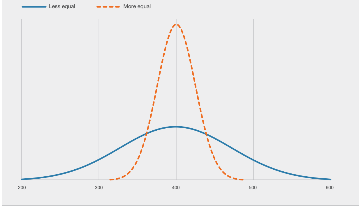
Figure 3.1 Hypothetical test score distributions with varying levels of inequality
