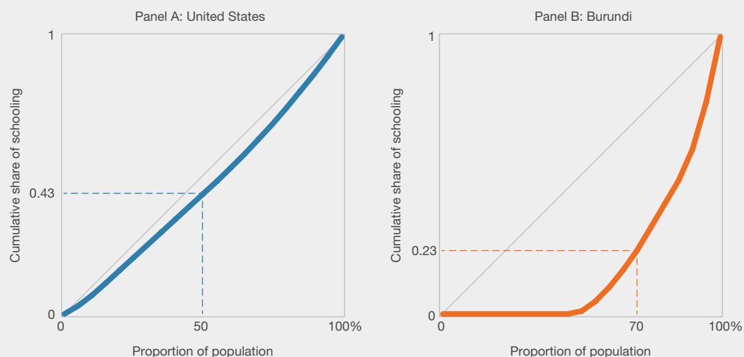
Figure 3.6 Lorenz curves for years of schooling in the United States and Burundi
