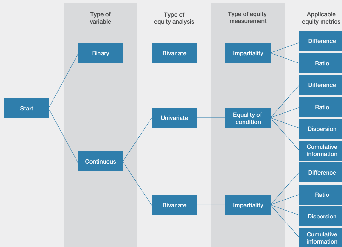
Figure 3.7 Decision tree for equity analysis and applicable metrics
