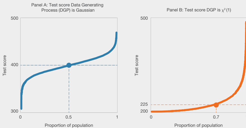
Figure 3.3 Hypothetical cumulative distributions under different distributional assumptions
