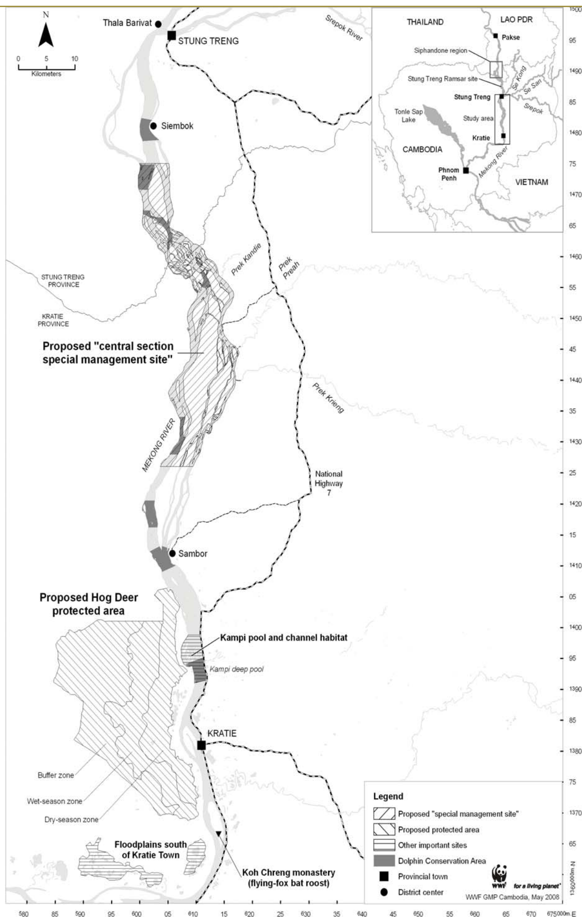
Figure 10. Priority sites for biodiversity conservation in the study area.
